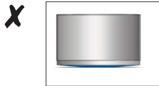
Figure 13 Pan base is bowed out and is NOT FLAT. Unit efficiency will be dramatically reduced during cooking. It may not even be detected.
