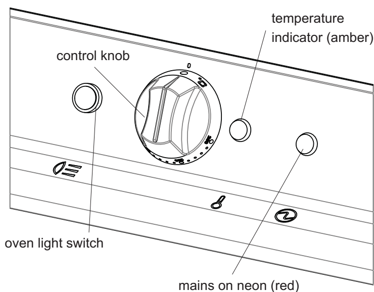
Figure 3 - Oven control
